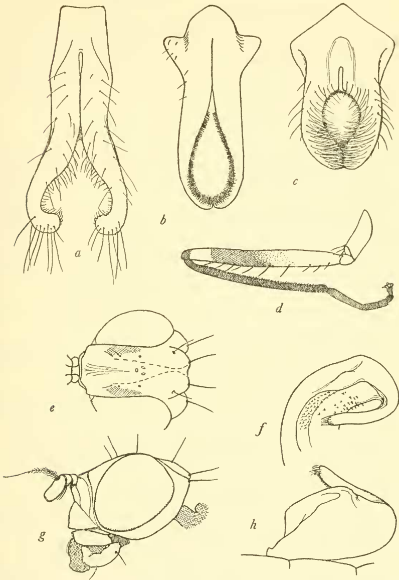
FIGURE 72.— a , Grammicomyia halli , new species, copulatory fork. b , Mimegralla perfulva , new species, copulatory fork. c , d , Townesa spinosa , new species: c , Copulatory fork, d , posterior aspect of left fore leg of male. e – h , Mimomyrmecia tessellata Frey: e , Dorsal aspect of head, f , ventral aspect of half of copulatory fork, g , lateral aspect of head, h , lateral aspect of copulatory fork.
